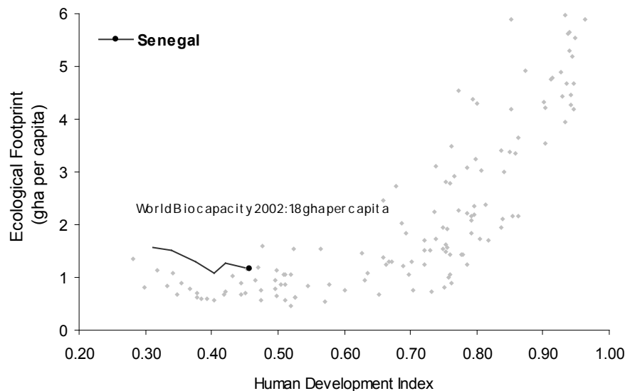
Figure 9.2.1: Human Development and Ecological Footprint of Nations, HDI Time Trend Line from 1975 - 2003
